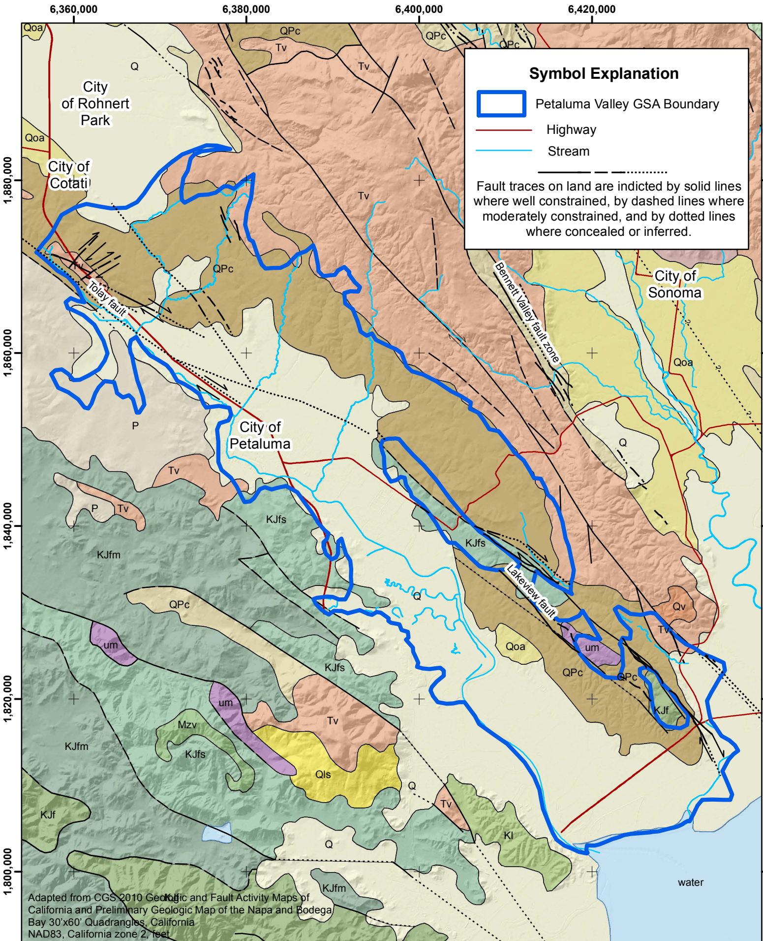
Petaluma Valley GSA Geologic Map
